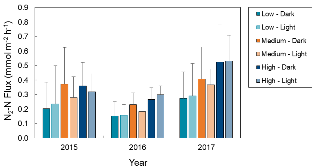
Figure 3. Sediment-water efflux of \text{N}_2\text{-N} from whole-community incubations for low, medium, and high oyster densities. Averages ( \pm std. dev.) of both dark and light incubations for all May–October incubations are presented.
