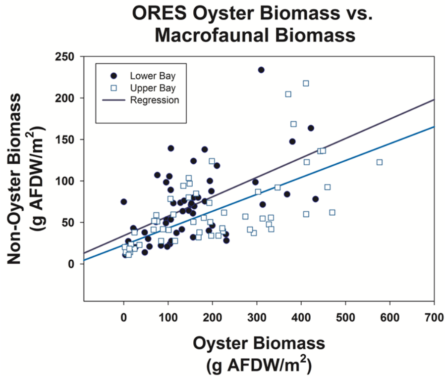
Figure 10. Relationship between oyster biomass and non-oyster macrofaunal biomass with linear regression lines from two studies, lower Chesapeake Bay (filled circles, dark blue line) and upper Chesapeake Bay (open squares, light blue line). Using log-transformed data, regression lines differed significantly by lower vs. upper Bay (General Linear Models and Aikaike's Information Criterion), presumably driven by the overall salinity gradient.
