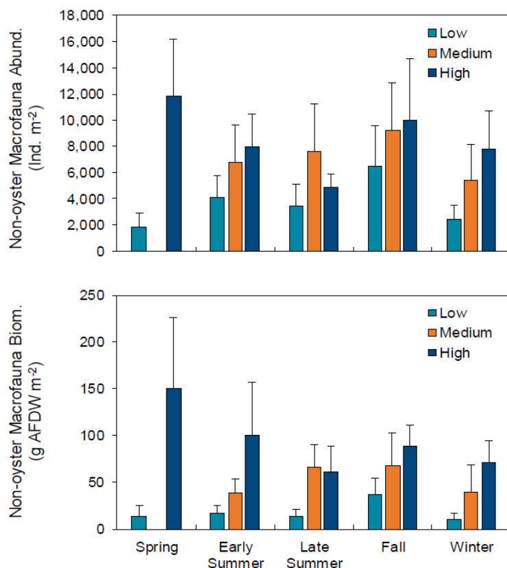
Figure 8. Seasonal non-oyster macrofaunal abundance and biomass density relative to low ( < 50.0 \text{ g DW m}^{-2} ), medium ( 50.0\text{--}224.9 \text{ g DW m}^{-2} ), and high oyster density ( \geq 225.0 \text{ g DW m}^{-2} ). In spring, none of the samples collected fell in the medium oyster biomass category. Error bars represent one standard deviation. Refer to text for results of statistical analyses of biomass data.
